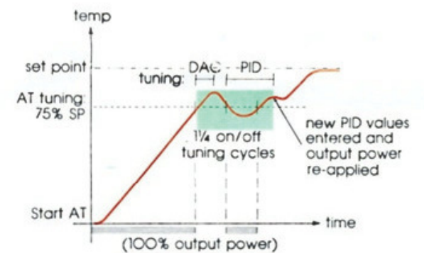
Fig. 1 Autotune AT
