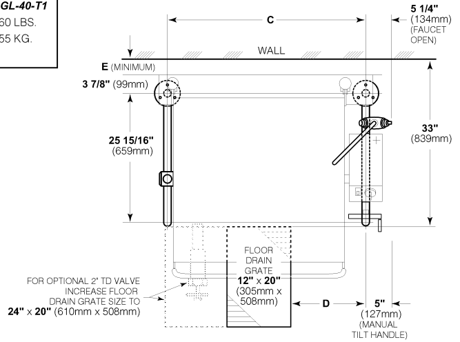
LEG LOCATION & SUGGESTED FLOOR DRAIN DETAIL
