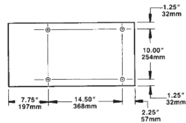
MOUNTING DIAGRAM TOP VIEW
