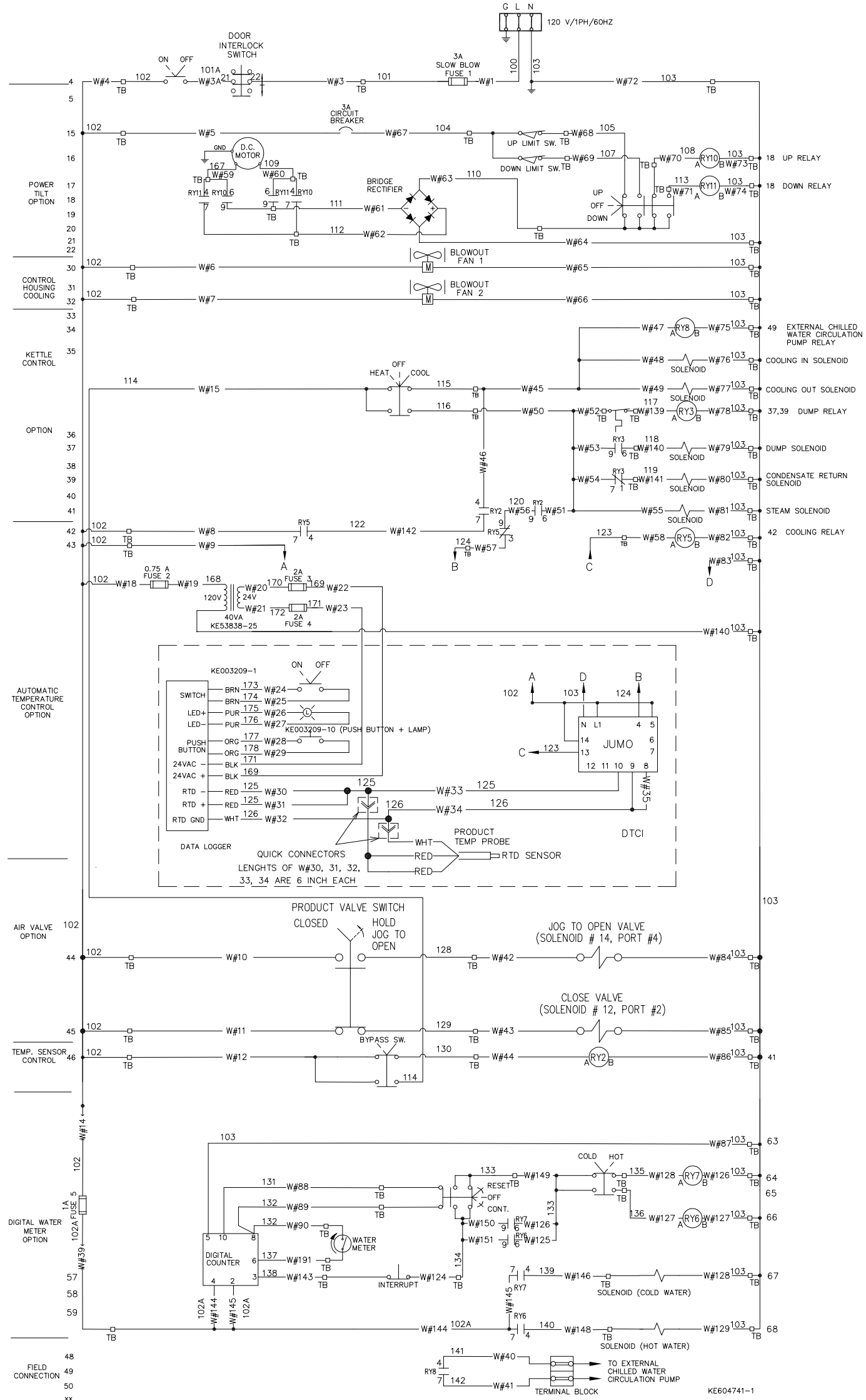
HA-MKDL-T or HA-MKDL-CC HEAT/COOL WITH CONTROL
