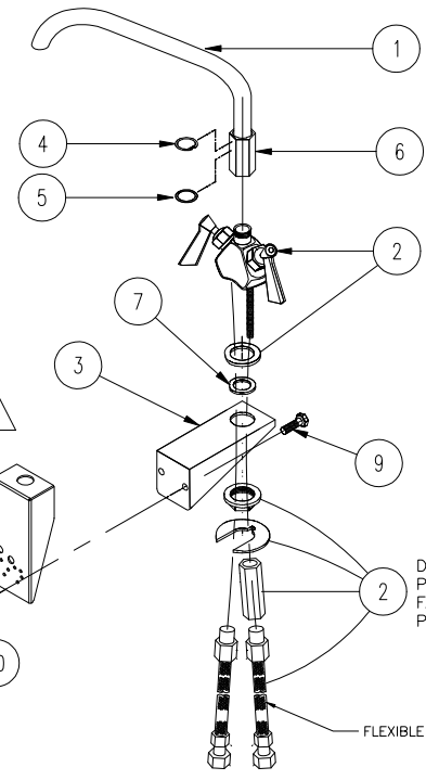
DETAIL A (DOUBLE PANTRY FAUCET MTG DETAIL)
