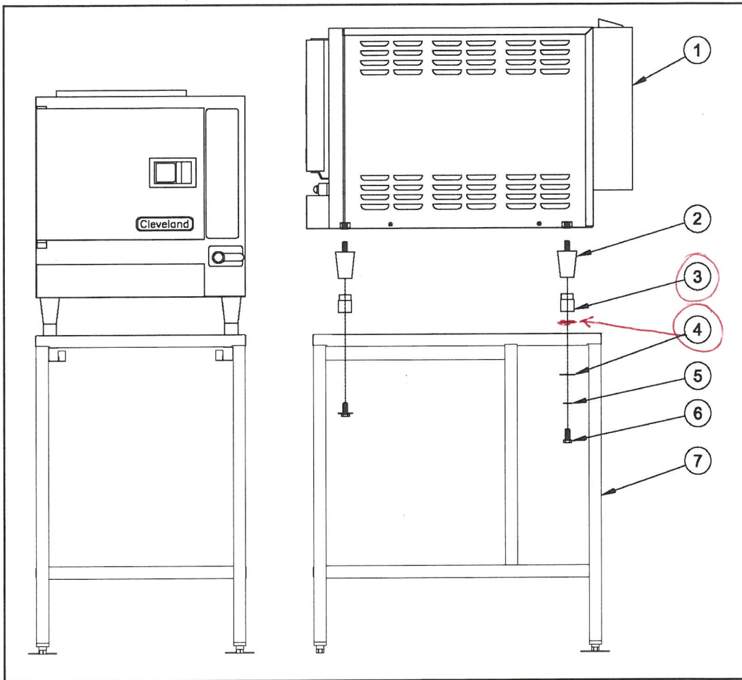
Figure 9 SteamChef™ GAS Mounting Instructions (Model 22CGT3 shown on Unistand34)
