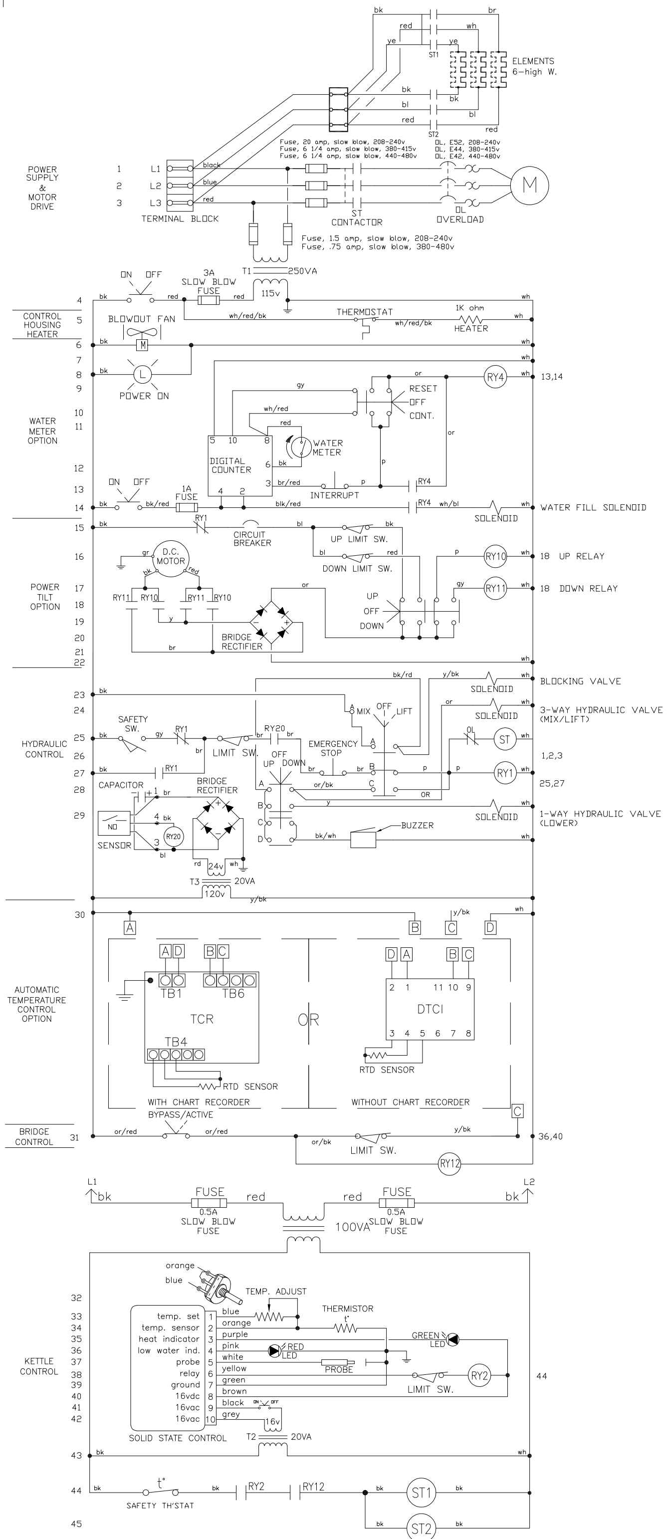
ELECTRIC MIXER KETTLE (ALL OPTIONS) 380-600 volts KE90417-6 V
