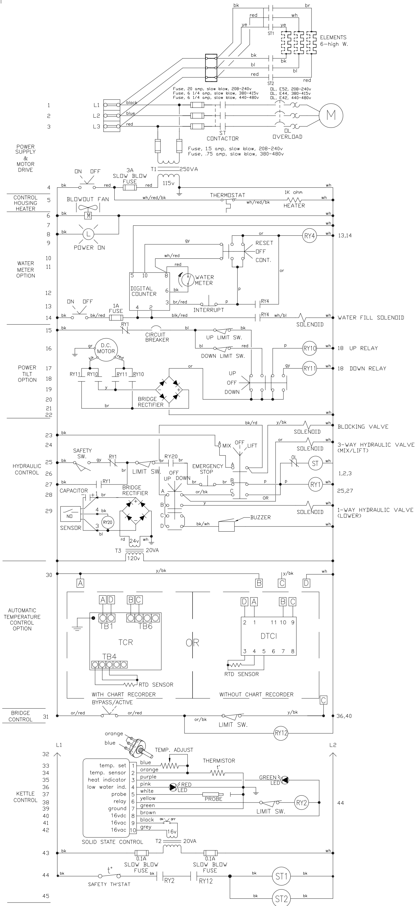
ELECTRIC MIXER KETTLE (ALL OPTIONS) 208-240 volts
