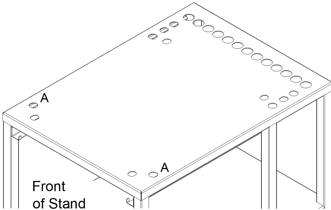
Figure 1 SteamCraft® Mounting Holes
