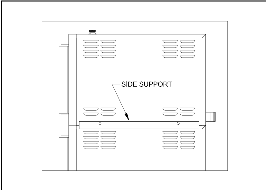
Figure 3 Side Support Attachment
