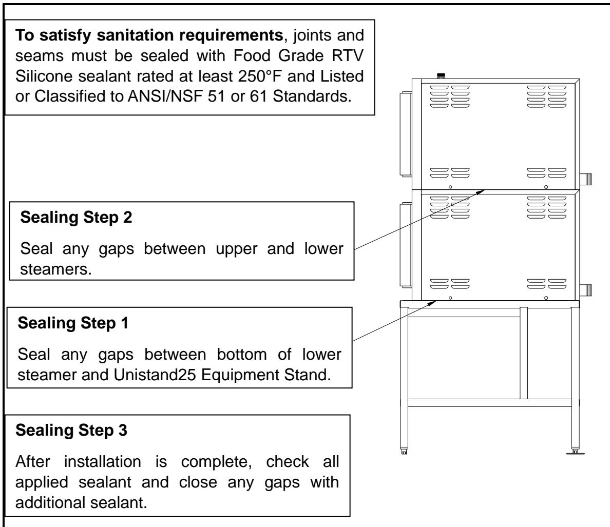
Figure 2 Sealing Requirements
