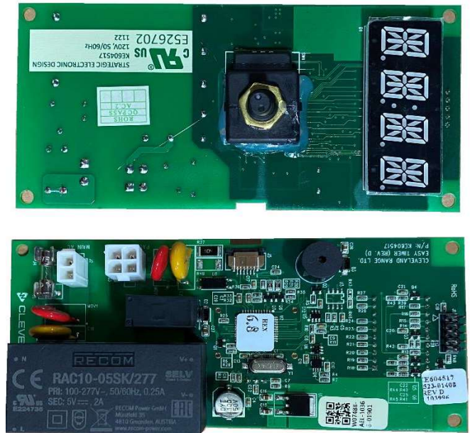
KE604517 EasyTimer PCB
