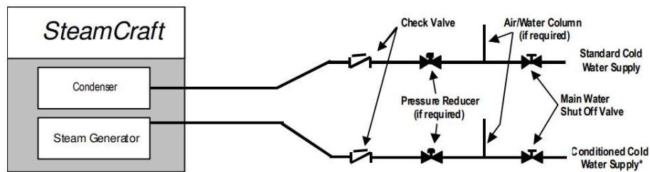
Figure 3-5 Cleveland Range Separate Water Supply Arrangement when Using Separate Conditioned* Feed Water Supply
