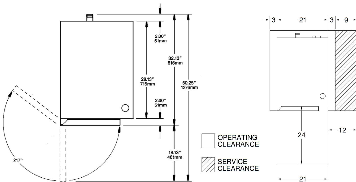
Figure 2-2 SteamCraft Electric – Front-, Back-, and Right-Side View Dimensions (Model 21CET16)
