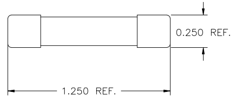
STYLE B FUSE HOLDER KE51139
