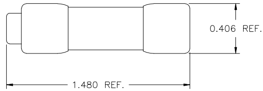
STYLE A FUSE HOLDER KE51139-1
