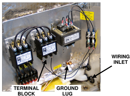
Figure 3-14 Electrical Connections
