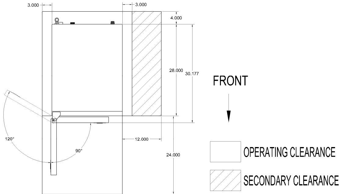
Figure 2-2 SteamChef 6.1 Dimensions and Clearances
