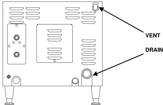
Figure 3-7 Steam Vent (SteamChef™ 3.1 Shown)
