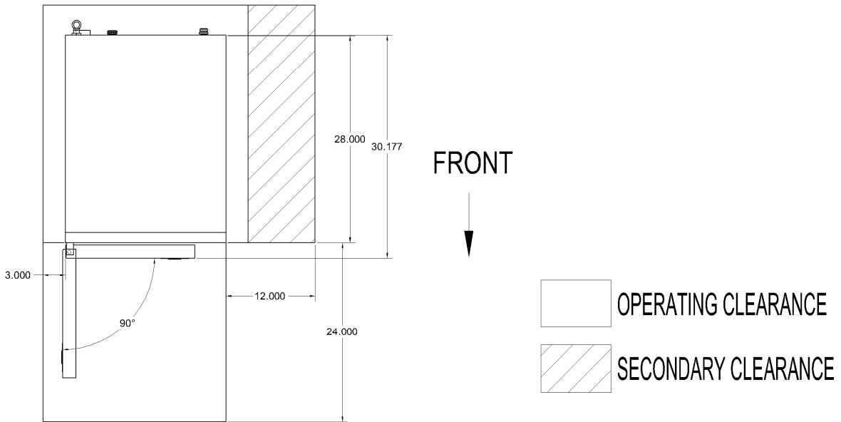
Figure 2-1 SteamChef 3.1 Dimensions and Clearances
