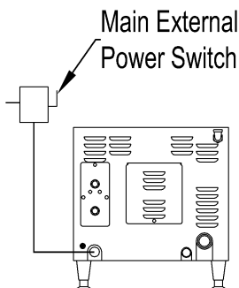
Figure 3-12 Electrical Layout
