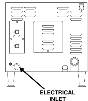
Figure 3-13 Electrical Connection Inlet
