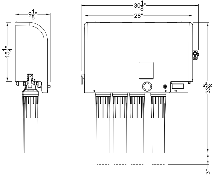
Water Processor Assembly - 120V
