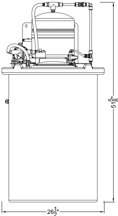
Re-pressurization/Storage Tank Assembly
