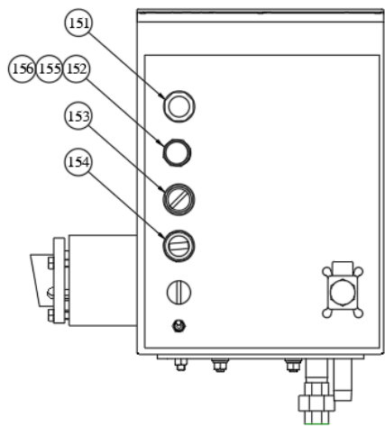
GEAR BOX ASSEMBLY W/NO WATER METER OPTION
