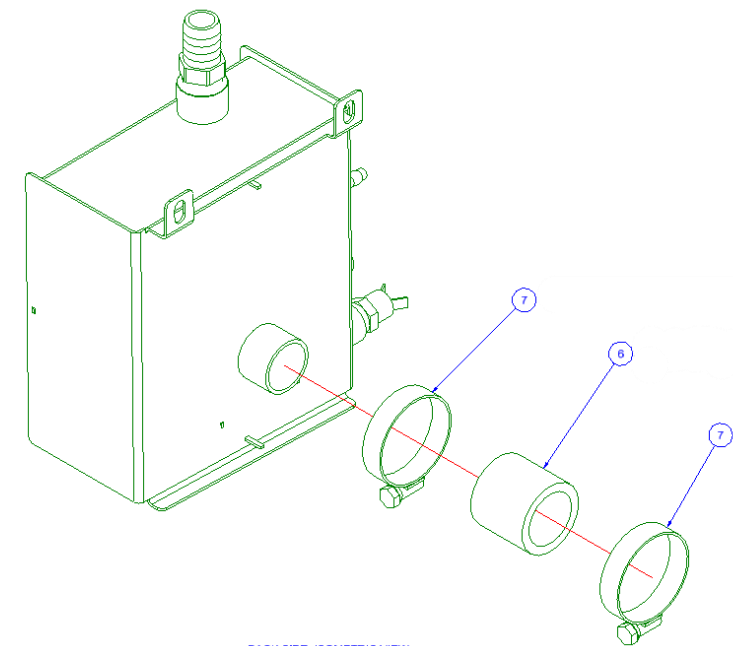
BACK SIDE, ISOMETRIC VIEW
