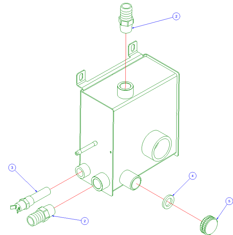
FRONT SIDE ISOMETRIC VIEW
